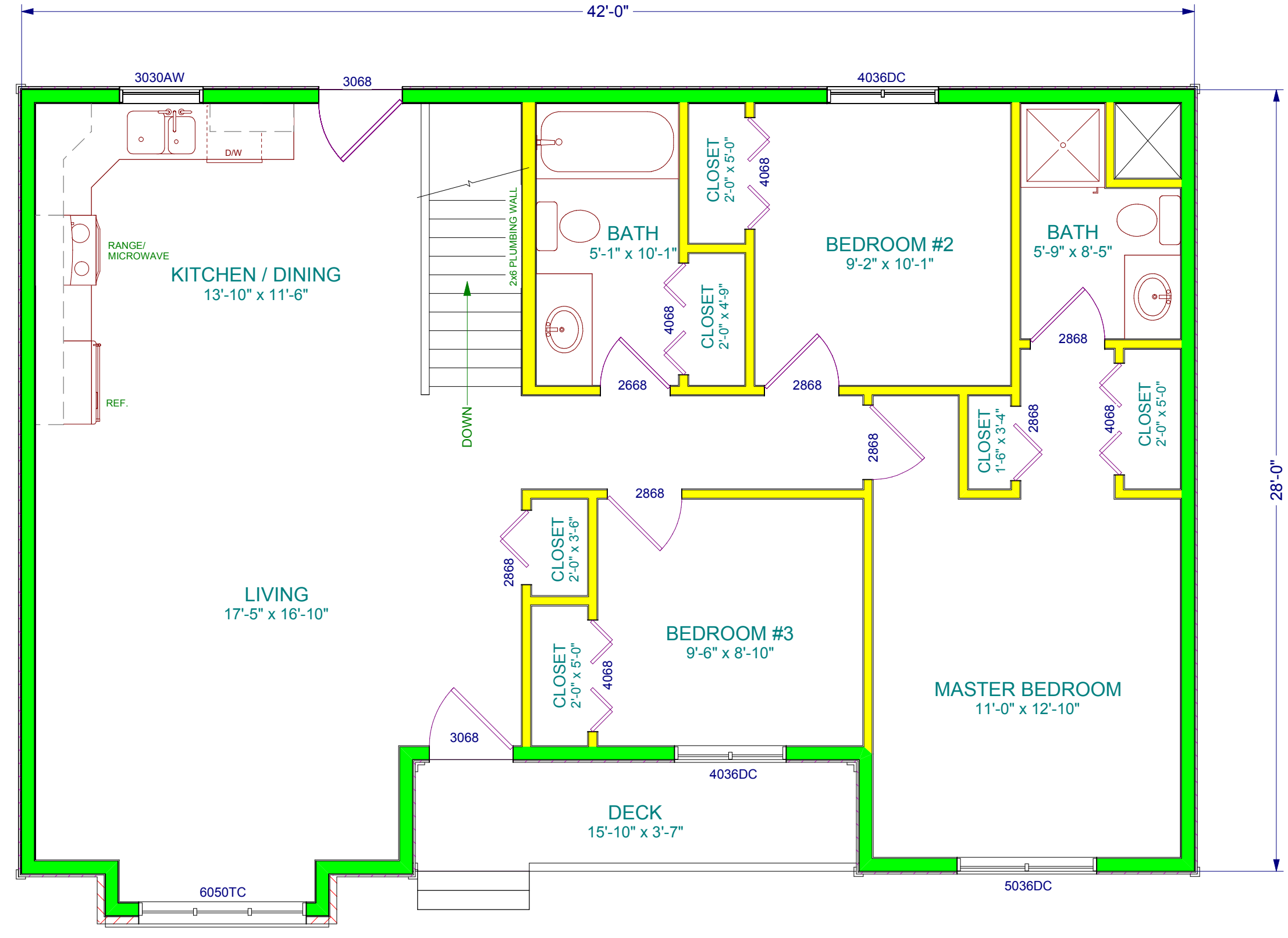
MAIN FLOOR PLAN SCALE: 1/4" = 1'-0"
