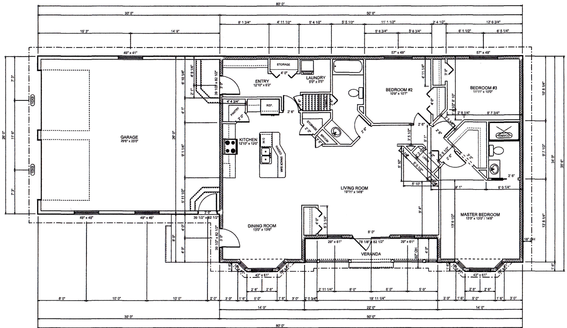
MAIN FLOOR PLAN HOUSE 1832 SQ. FT. GARAGE 780 SQ. FT.
